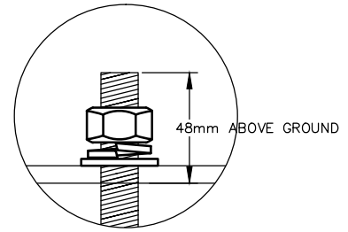
FIXING DETAIL
